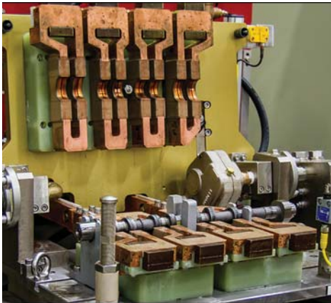
Fig. 3. CamPro™ machine utilizes patented non-rotational hardening technology (SHarP-C™ technology)
